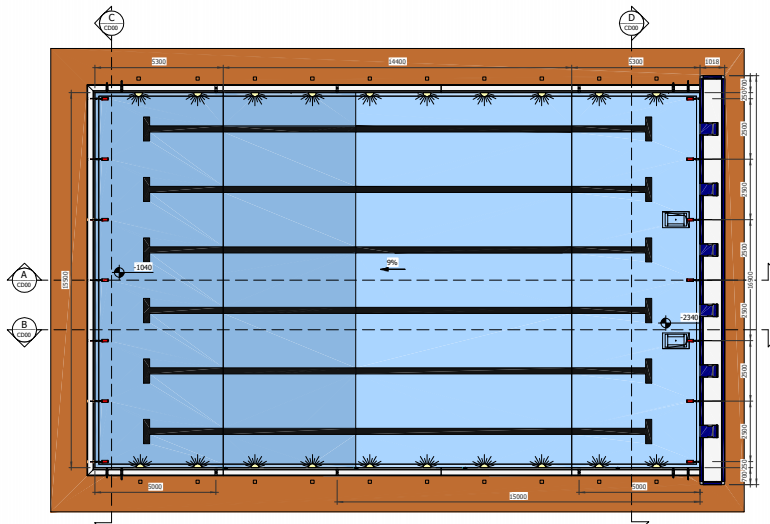
POOL PLAN VIEW Scale 1 : 100
